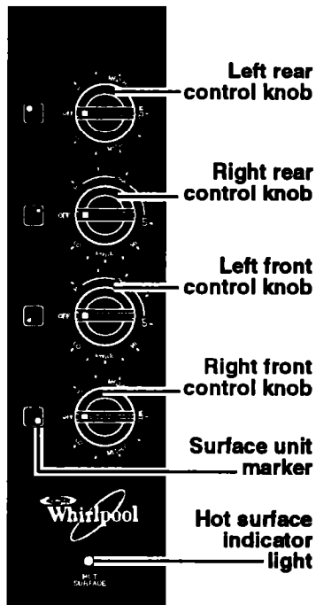
Dual element control panel (Model RC8640XB)
